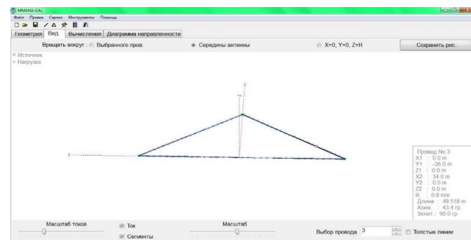
Figure 4. The image of Delta Loop antenna in MMANA program.
