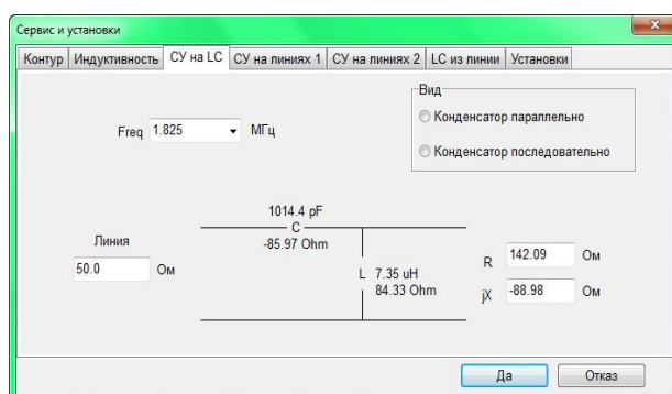
Figure 10. Delta Loop Antenna Adapter Parameters
