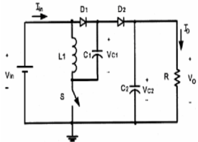
Figure 3.The basic circuit of LUO Converter.
