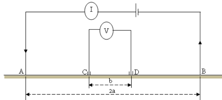
Figure 4: A typical Schlumberger electrode configuration.
