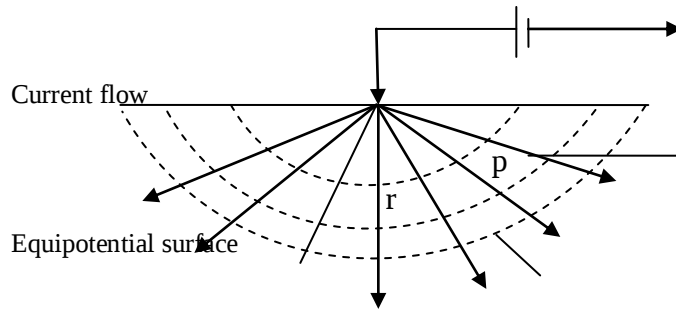
Figure 2: Current flow from a single surface electrode.
