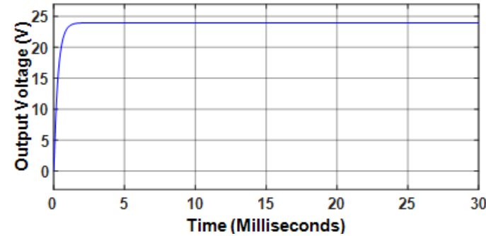
Fig. 8. Output voltage of PID controller for SEPIC when resistive load and constant input ( V_{in} , 17 V) are used
