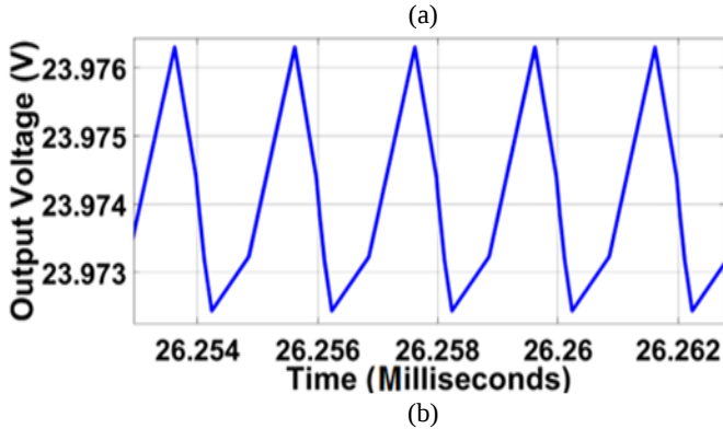
Fig. 7. Output voltage for the LLC (open loop design); (a) full waveform and (b) zoomed in
