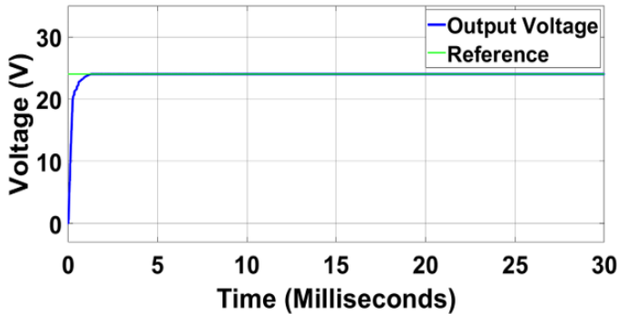
Fig. 12. Output voltage of SEPIC using FLC
