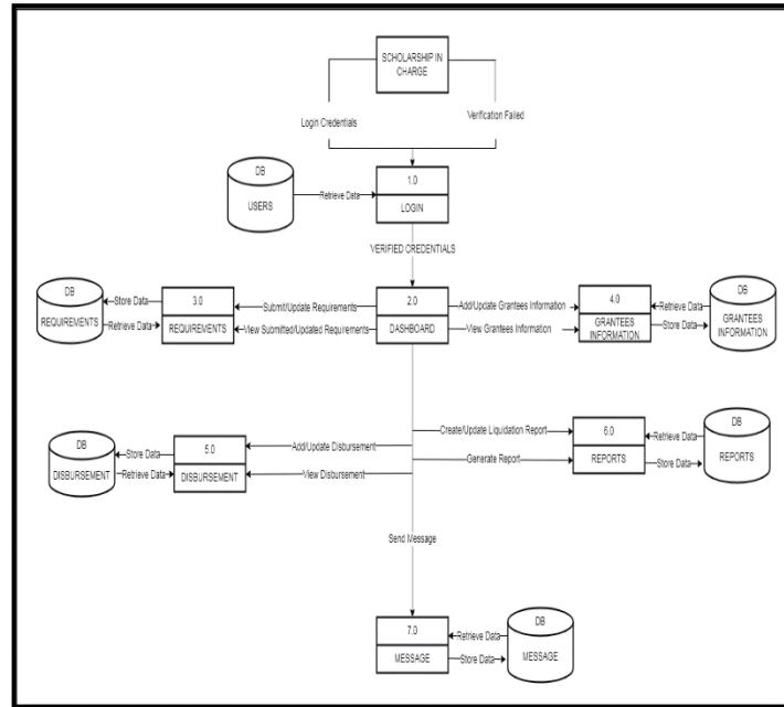
Figure 5. Context Diagram
