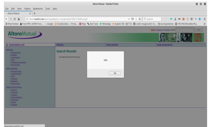
Fig. 3. Reflective XSS on AltoroMural Lab
