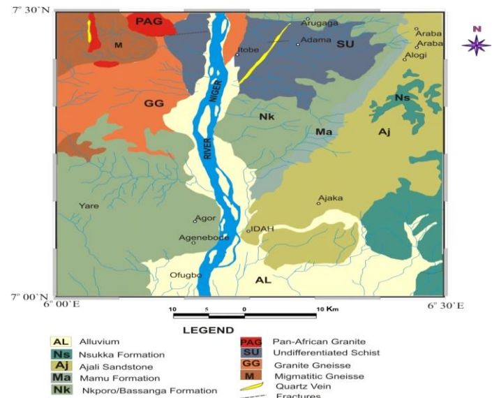
Fig. 1.0 Geology map of the study area after Obiora et. al., (2006)
