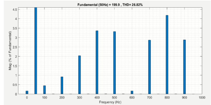
Figure 10 FFT analysis of five level inverter
