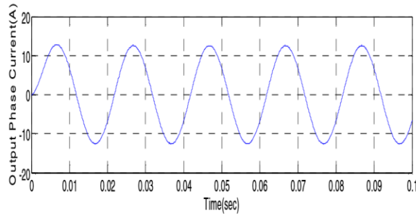
Figure 7 : Current
