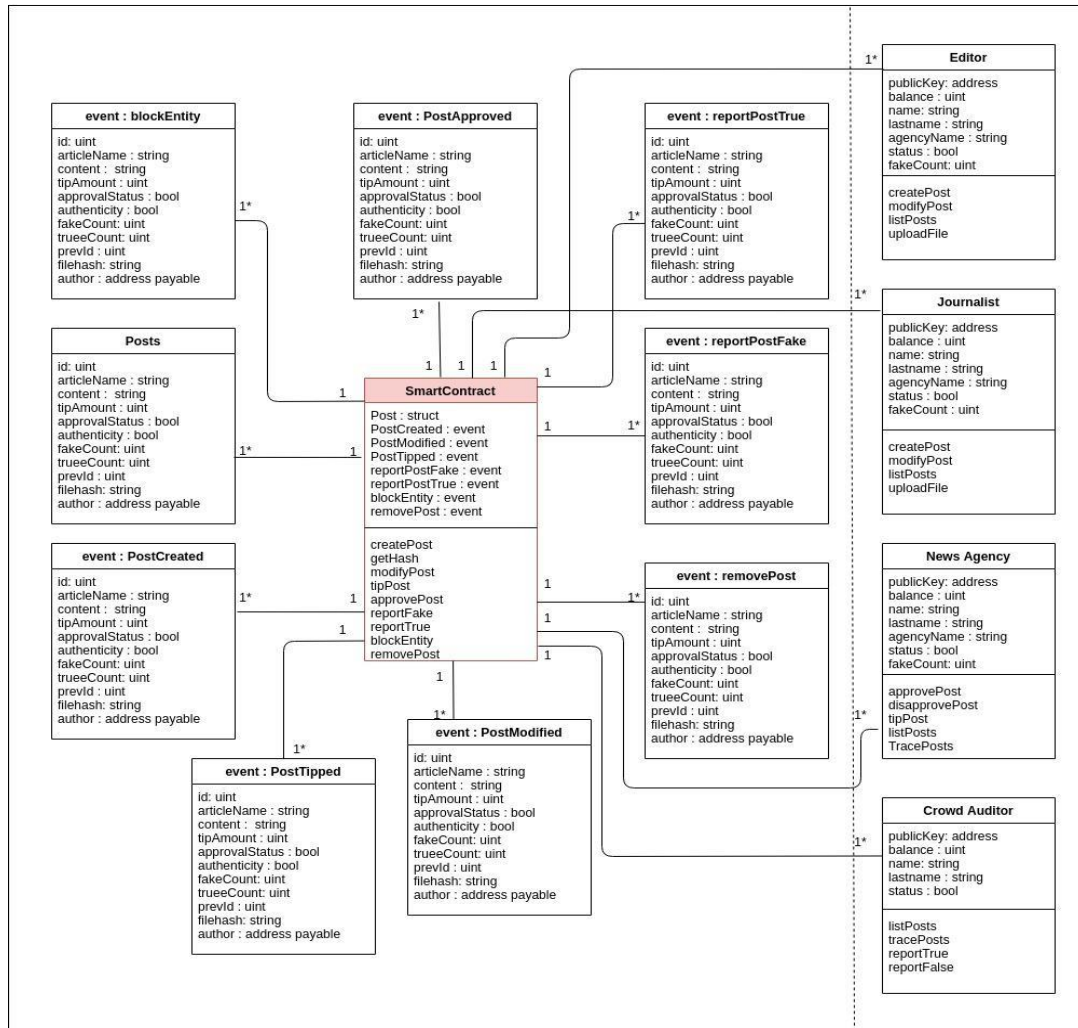
FIGURE 4. UML Diagram
