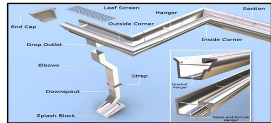
Figure 2: Typical Gutter used in RWHS
