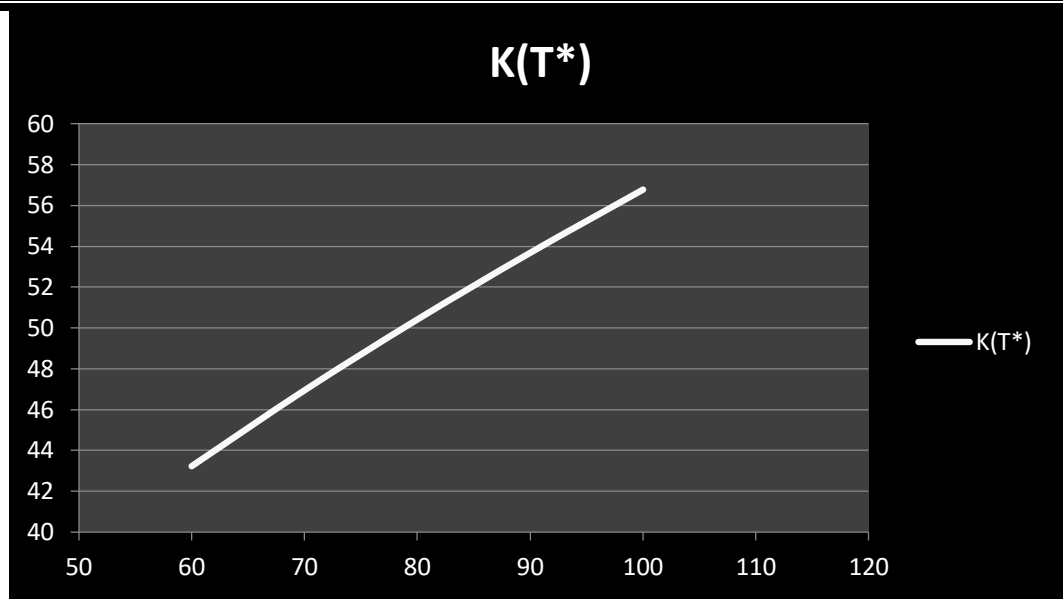
Fig. 4: Impact of C_2 on K(T^*) : Crisp model
