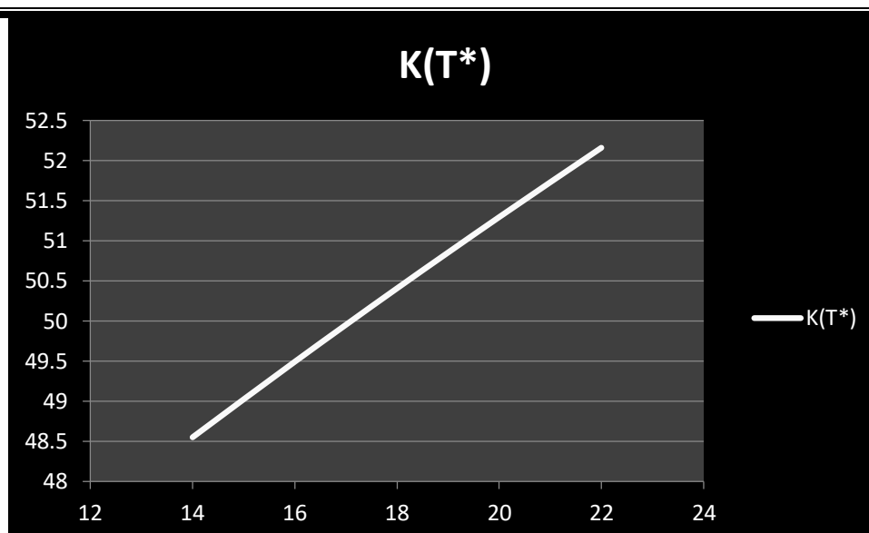
Fig. 8: Impact of C on K(T^*) : Crisp model
