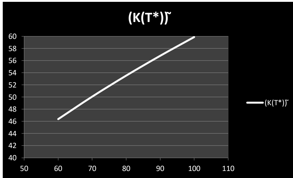
Fig. 5: Impact of C_2 on \widetilde{K(T^*)} : Fuzzy model
