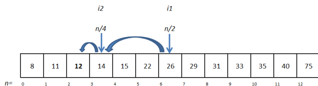
Fig. 3. : Binary Search- Example
