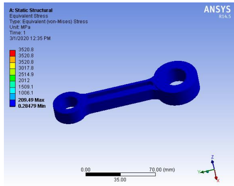
Fig. 13. Equivalent Stress
