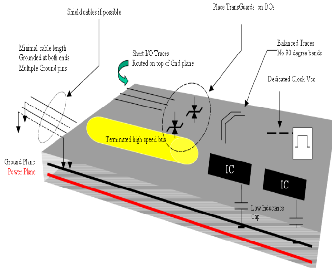
Fig.3 Ground plane added to PCB
