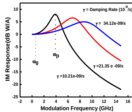
Fig. 2. Simulated modulation response of 1.55µm DFB laser for direct current modulation above threshold.
