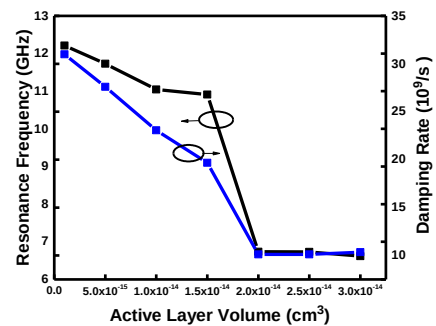
Fig. 7. Measured resonant frequency and damping rate against the active layer volume.
