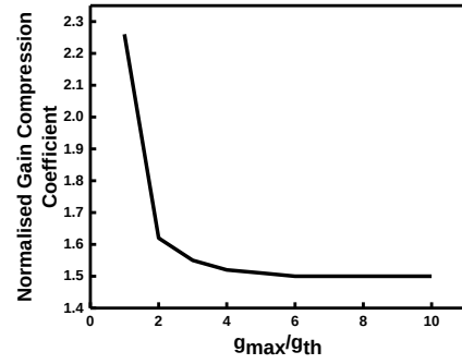
Fig. 6. Calculated normalized gain compression against the gain ratio.
