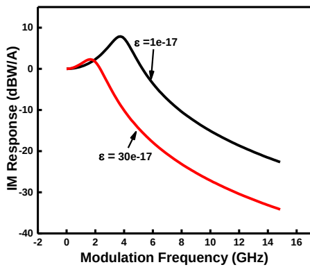
Fig. 5. Effect of gain compression on the IM response.
