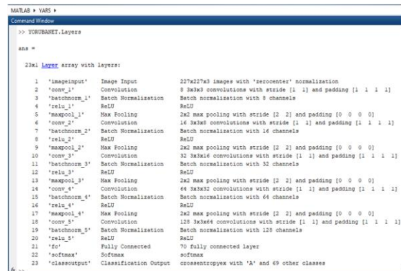
Figure 2: YORUBANET Architecture
