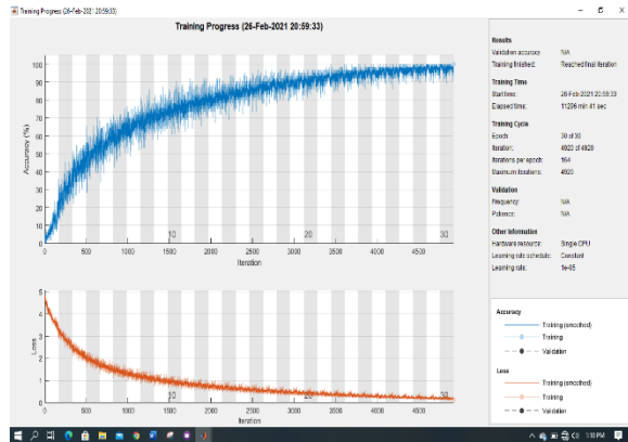
Figure 3: Training Progress
