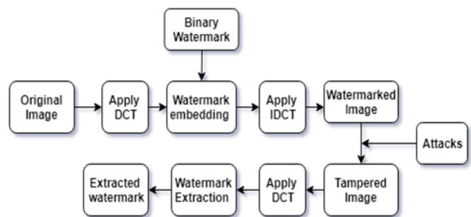
Fig 2. Block diagram of Digital Image Watermarking using DCT
