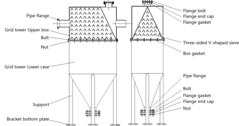
Fig. 2. Overall structure of the sieve tower
