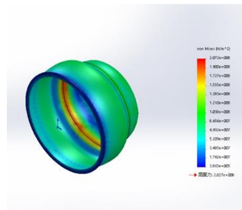
Fig. 12. Upper cylinder stress cloud diagram
