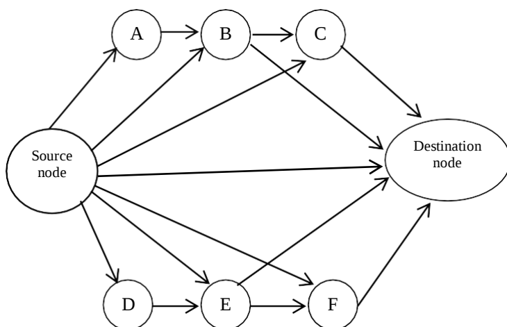
Fig 3: Route Discovery
