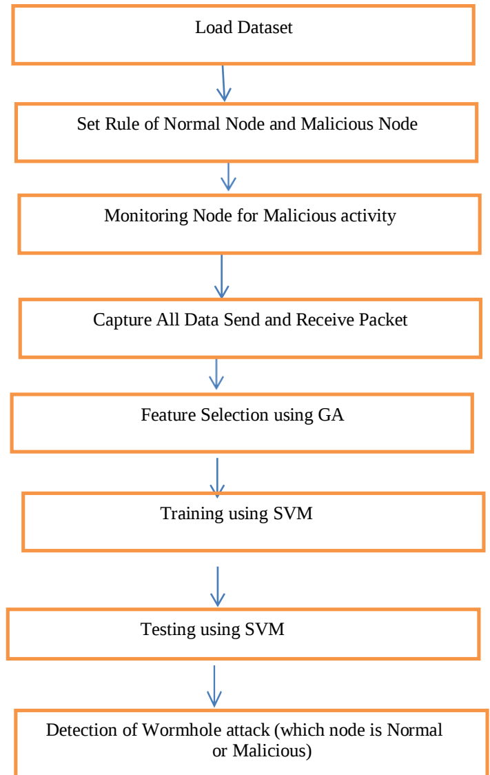
Fig 4: Proposed Methodology
