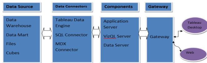
Fig 3. Tableau Architecture
