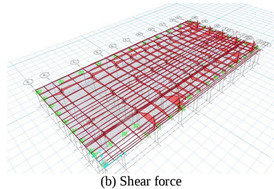
Figure 12: Bending moments and Shear force due to Live loads in both layers Table 9 gives the detail of bending moments and shear forces in the strips of the raft slab.
