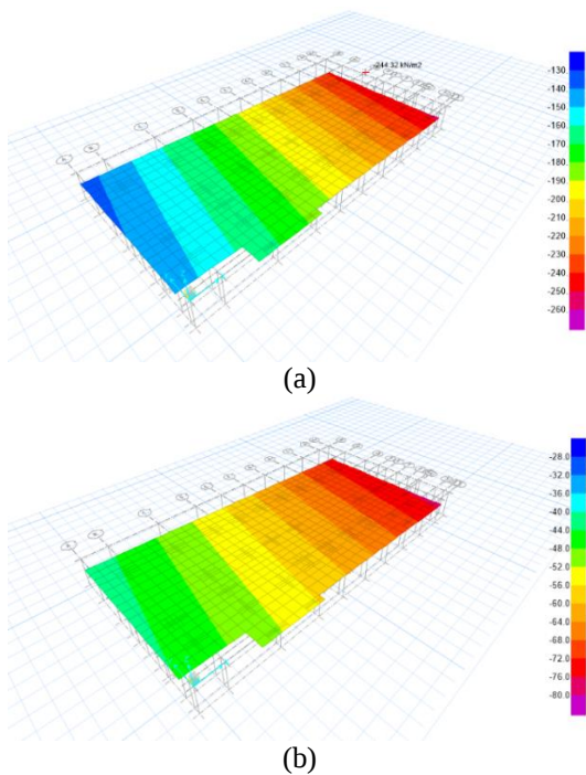
Figure 11: Results for (a) Soil pressure on raft slab, (b) Displacements of deformed raft Table 8 presents the displacement values of the raft slab due to dead load and live load.
