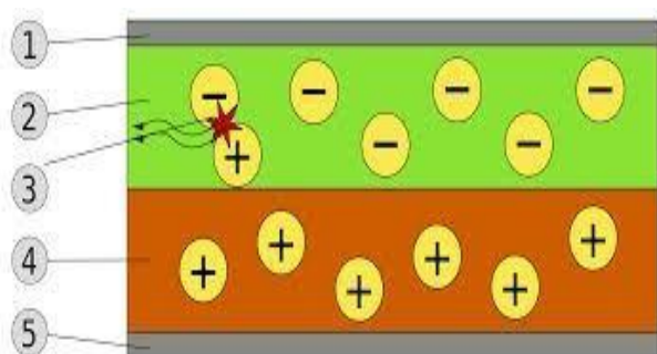
Fig. 2: Bilayer Oled: 1. Cathode (-), 2: Emissive Layer, 3: Emission Of Radiation, 4: Conductive Layer, 5: Anode (+)
