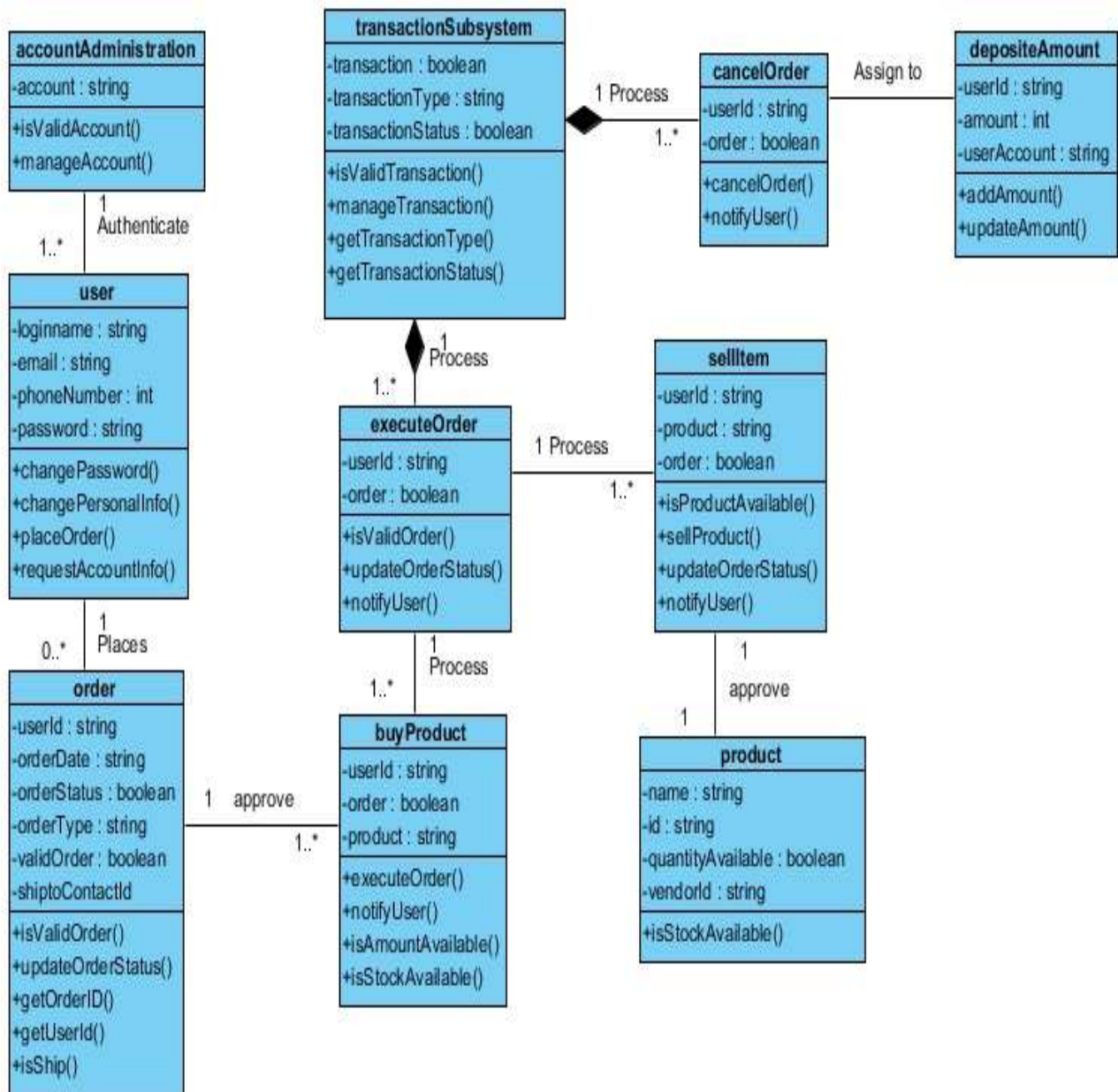
Fig 1: Class Diagram of Online Shopping System
