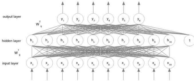
Fig. 1. An example of auto-encoder
