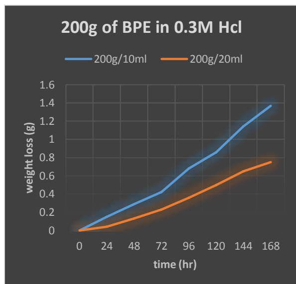
Figure 1: Graph of weight loss against time both in H_2SO_4 and HCl of different weight of BPE.
