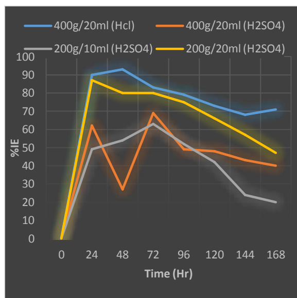
Figure 2: Graph of % IE against time at different concentration in HCl and H_2SO_4
