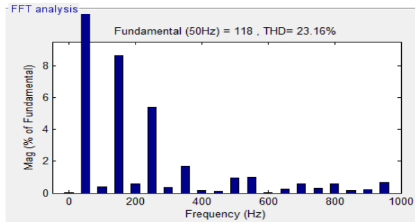
Fig 9. Phase voltage THD for three phase MLI
