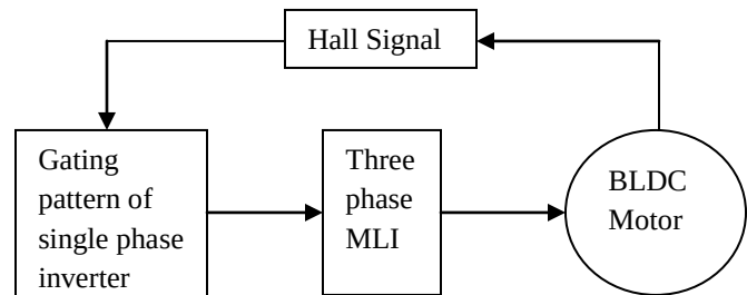
Fig 3. Sensored control of three-phase ANPCMLI fed brushless DC motor.
