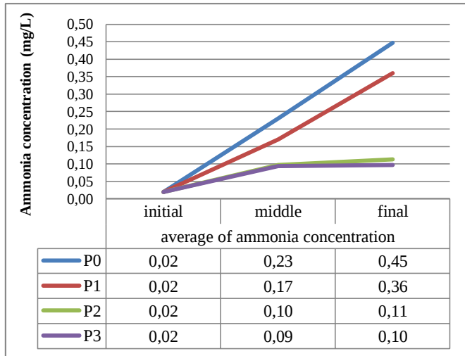
Figure 3. Ammonia concentration ( \text{NH}_3 ) in the treatment tanks.
