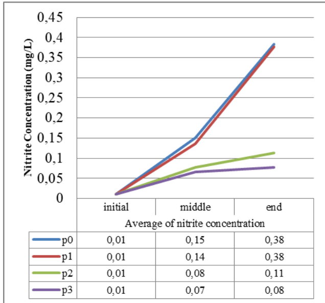
Figure 5. Nitrite concentration ( \text{NO}_2 ) in the treatment tanks
