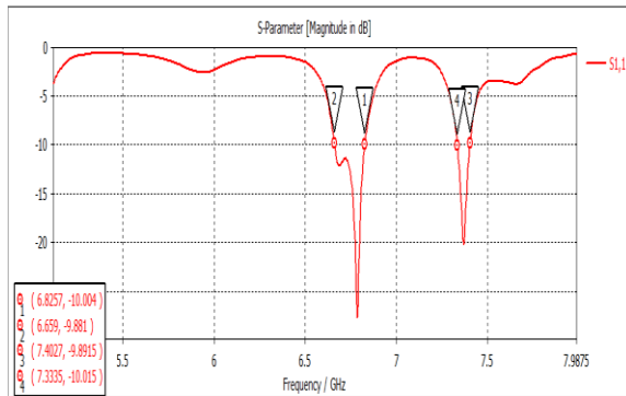
Fig 3. Return loss [S11] of triangular patch antenna
