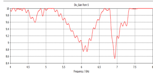
Fig 7: Diversity Gain of triangular patch antenna
