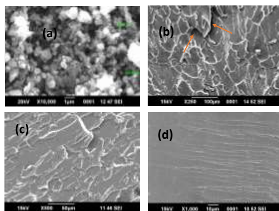
Figure 3.4 SEM image of (a) Nano NiO and tensile fractured surface of (b) neat UPR composite (c) UPR/N5 (d) UPR/NA3
