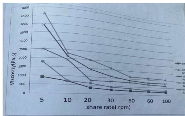
Fig. 2. Effect of shear rate on the viscosity of SAP pastes from native starch. Starch: Albumen of 5:95 (5 % NS), 10:90 (10 %NS), 15:85 (15 % NS), 20:80 (20 % NS), 100% EW, NS= Native starch, EW= Egg white
