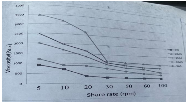
Fig. 2. Effect of shear rate on the viscosity of SAP pastes from acid modified starch. Starch: Albumen of 5:95 (5 % AS), 10:90 (10 %AS), 15:85 (15 % AS), 20:80 (20 % AS), 100% EW, AS= Acid modified starch, EW= Egg white
