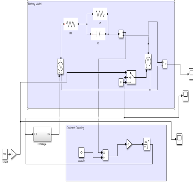
Fig.4 Simulink Block Diagram of Thevenin's Model
