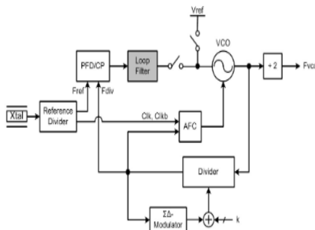
Fig.3. Fractional-N Synthesizer Based On AFC
