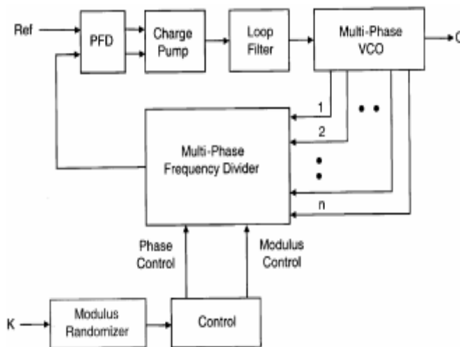
Fig.4. Multiphase VCO Fractional-N Synthesizer
