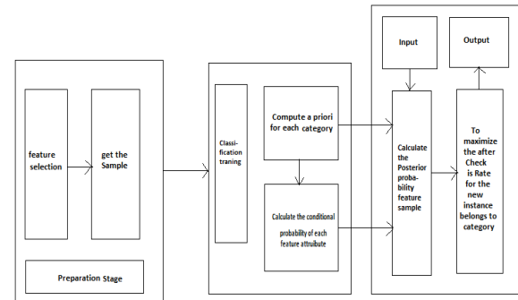
Fig. 4 Naive baye's network traffic identification process
