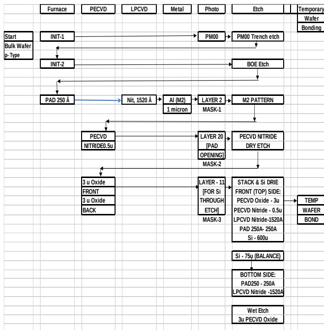
Fig. 7. Process Flow for fabrication of interposer.
