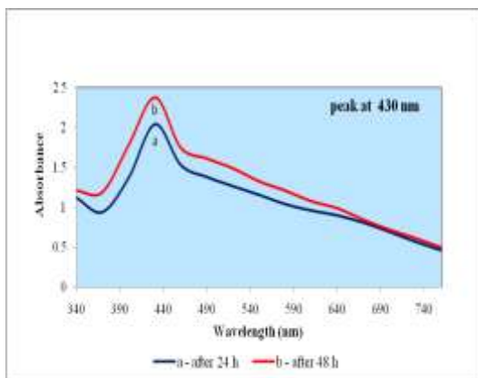
Fig 2. UV-vis spectra of reduction of Ag ions to Ag nanoparticles
