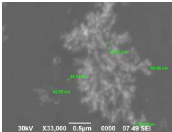
Fig 4. SEM image of Ag nanoparticles
