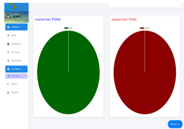
Fig 4 : Data Visualization
