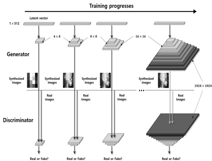
Figure2: Conceptual Architecture of PPGAN
