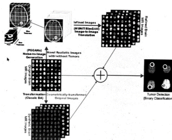
Figure1: Better tumor detection can be achieved by combining noise-to-image and image-to-image GANs: the PGGANs independently produce several realistic brain tumor/non-tumor MR images, the MUNIT independently refines them, and the binary classifier uses them as extra training data.
