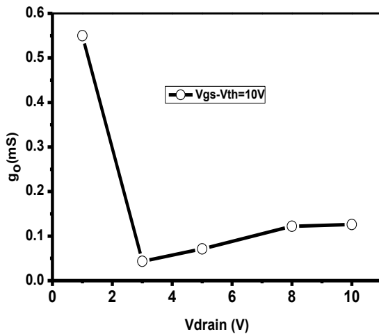
Fig. 7. Out put conductance at V_{gs}-V_{th}=10V with varying drain voltage.
