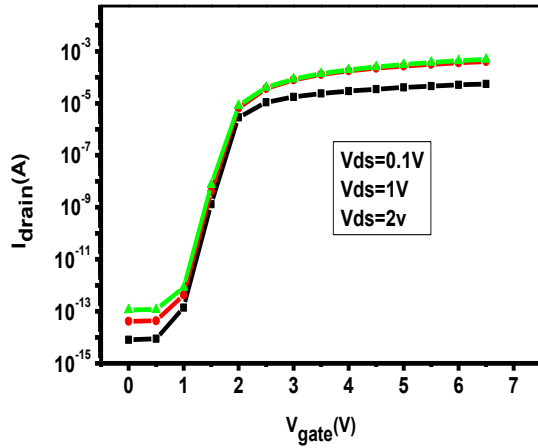
Fig. 4. Threshold voltage of LDMOS transistor .
