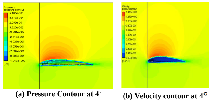
Figure 12: Pressure and velocity contours
