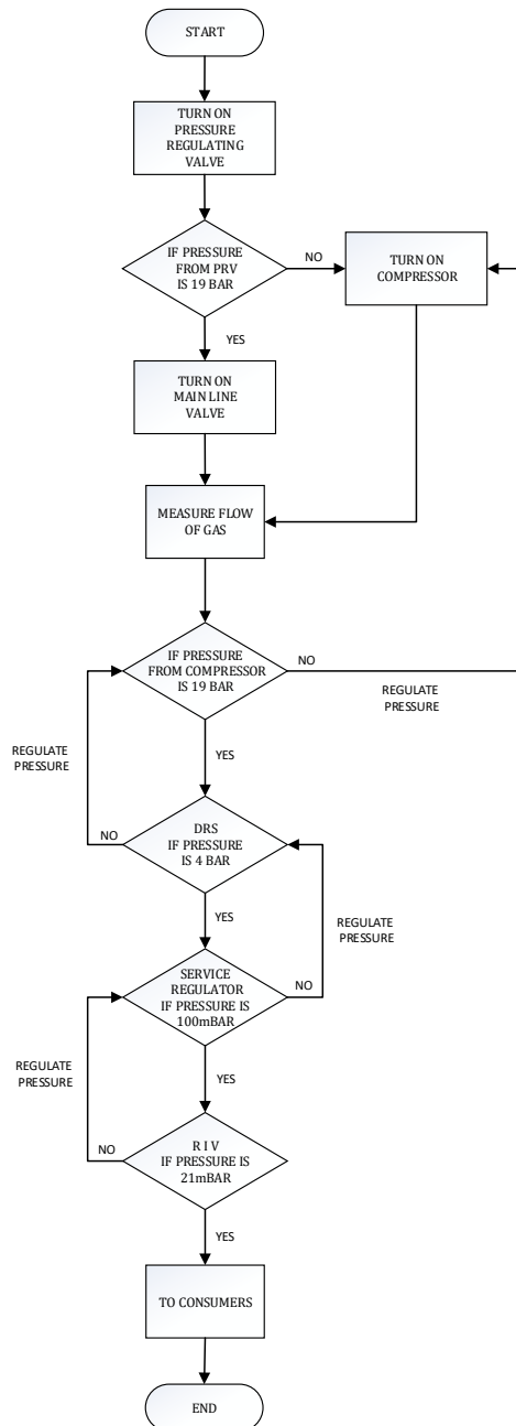
Fig.2 Process flow diagram of system
