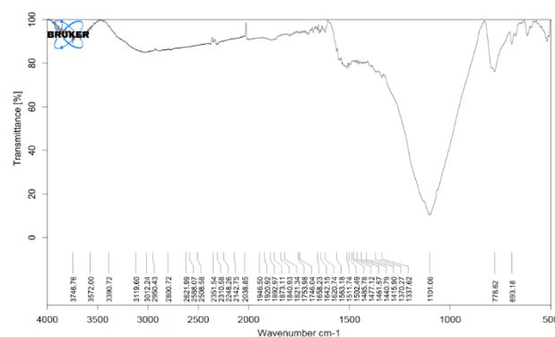
Fig 2. FTIR Analysis
