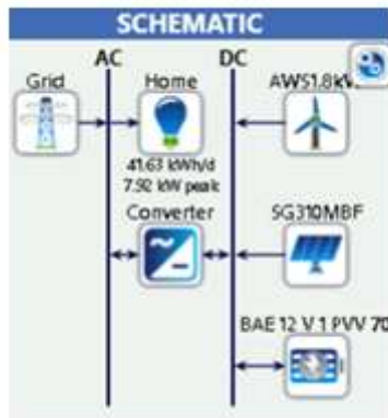
Figure 5. Schematic diagram for the proposed model in HOMER
