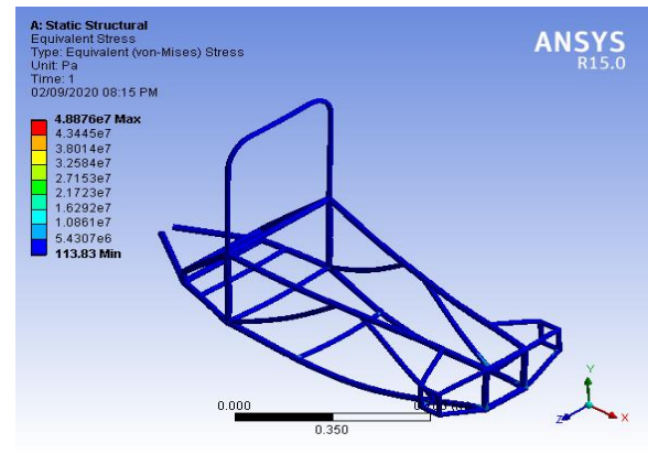
Fig.8. Von Mises stress for static loading
