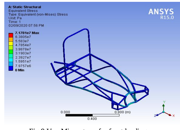
Fig.9. Von Mises stress for front loading
