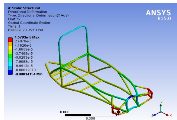
Fig.2. Front impact Analysis (Directional deformation)
