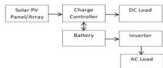
Fig. 1 Block Diagram of a Standalone Solar PV Home System
