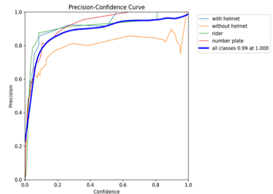
Figure 3: Precision-Confidence Curve
