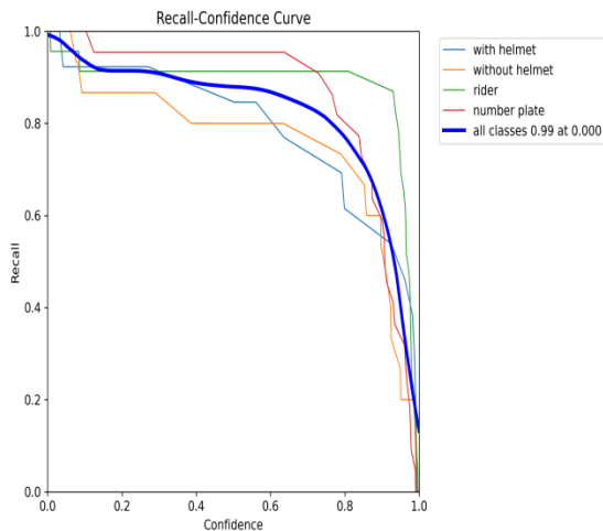
Figure 5: Recall-Confidence Curve
