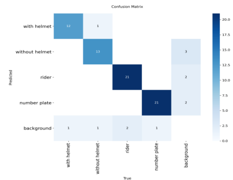
Figure 7: Confusion Matrix
