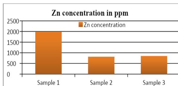
Figure 5: Zn in ppm in different sample type
