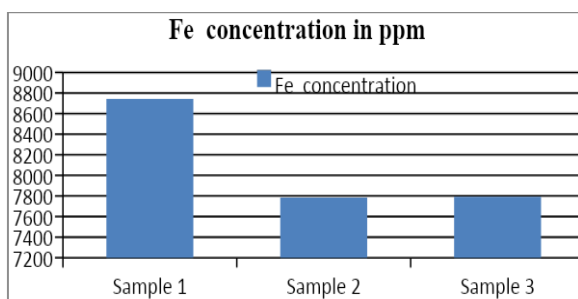
Figure 4: Fe in ppm in different sample type
