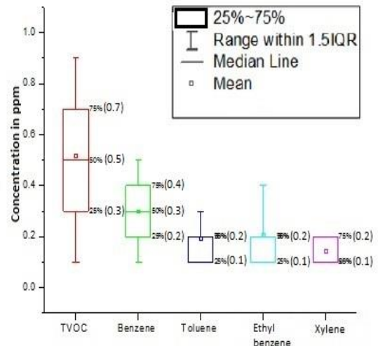
Fig.5. Graphical representation of variation in concentration of TVOC and BTEX at Bhagal Char Rasta (Morning) for Post-Monsoon
