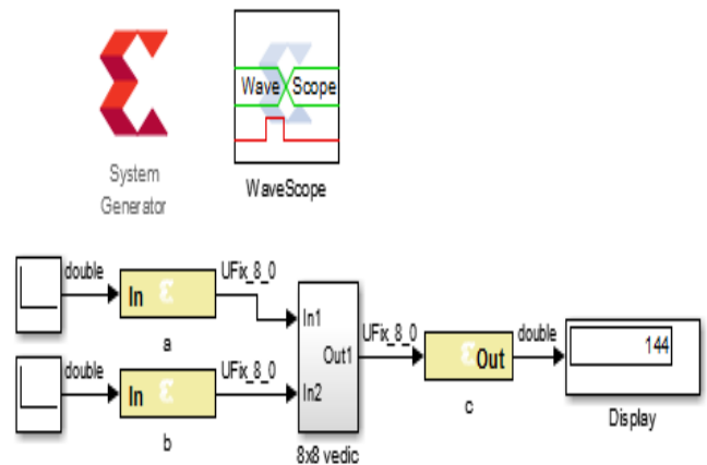
Fig 3: Fig. MATLAB Implementation of 8x8 Vedic Multiplier
