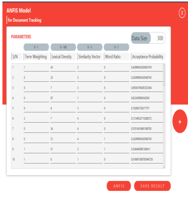
Fig. 4: Data Input Interface
