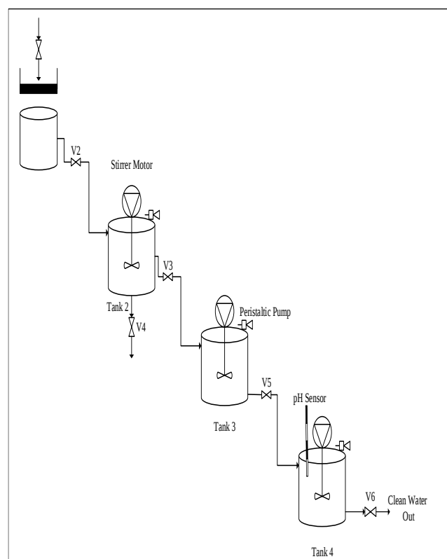
Figure 4: P&ID
